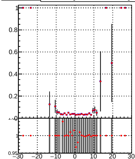
—•— DQM_TT_mkFit-DQM_time_orig2 —•— DQM_TT_mkFit-DQM_time_mod2
