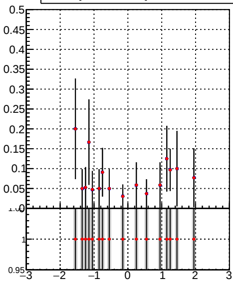
■ DQM_TT_mkFit-DQM_time_orig2 ● DQM_TT_mkFit-DQM_time_mod2
