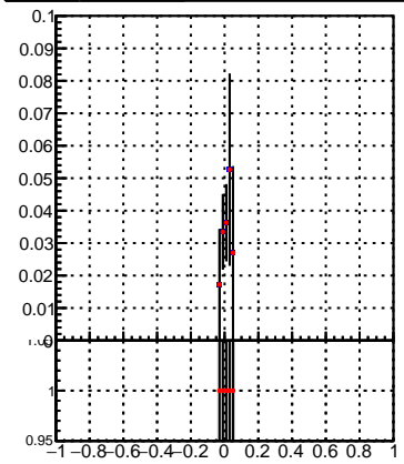
Efficiency vs Dxy(PV) - Legend: DQM_TT_mkFit-DQM_time_orig2 (black line), DQM_TT_mkFit-DQM_time_mod2 (red line)
