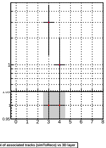
N of associated tracks (simToReco) vs 3D layer
