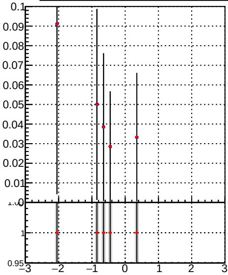
DQM_TT_mkFit-DQM_time_orig2 DQM_TT_mkFit-DQM_time_mod2
