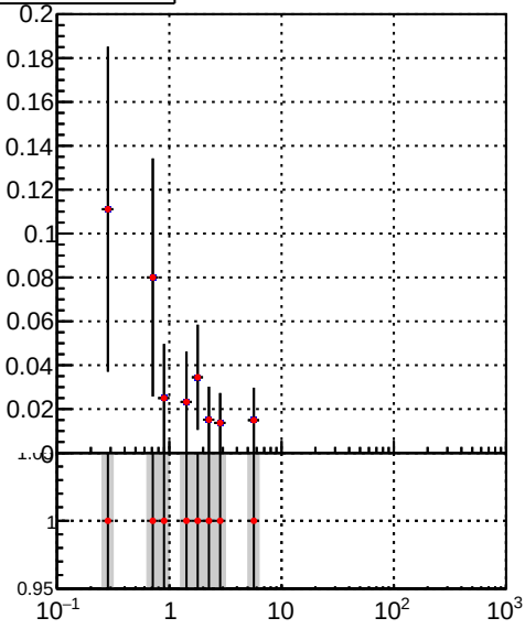
DQM_TT_mkFit-DQM_time_orig2 DQM_TT_mkFit-DQM_time_mod2
