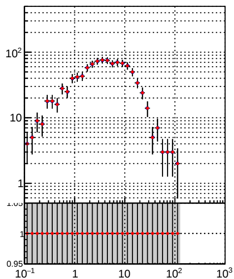
DQM_TT__mkFit-DQM_time_orig2 DQM_TT__mkFit-DQM_time_mod2
