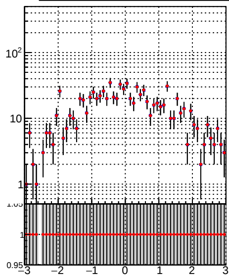
DQM_TT__mkFit-DQM_time_orig2 DQM_TT__mkFit-DQM_time_mod2
