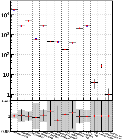
Number —●— DQM_TT__mkFit-DQM_time_mod2
