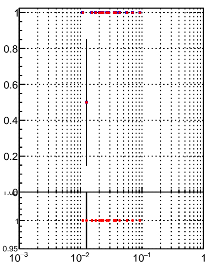
—●— DQM_TT_mkFit-DQM_time_orig2 -●- DQM_TT_mkFit-DQM_time_mod2
