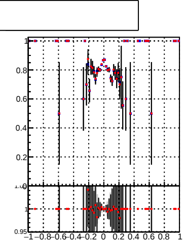
Pileup rate vs dz(PV)
