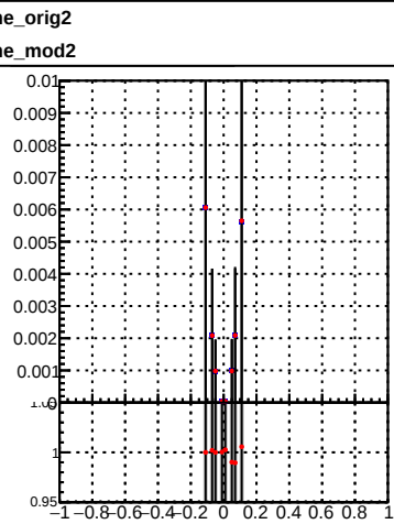
Duplicates Rate vs Dz(PV)
