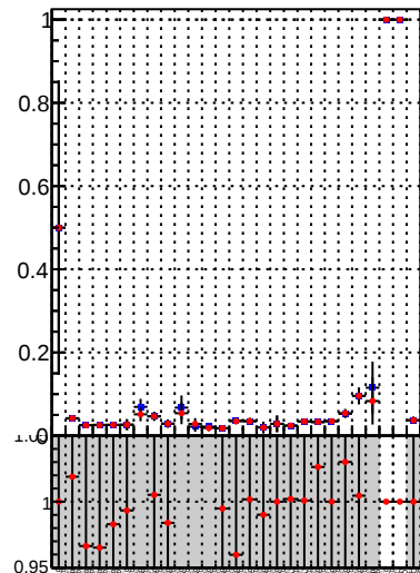
Fake rate vs. —•— DQM_TT_mkFit-DQM_time_orig2 —•— DQM_TT_mkFit-DQM_time_mod2
