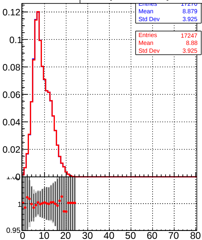
Legend: DQM_TT_mkFit-DQM_time_orig2 (grey histogram) DQM_TT_mkFit-DQM_time_mod2 (red histogram)
