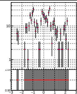
—●— DQM TT mkFit-DQM_time_orig2 —●— DQM TT mkFit-DQM_time_mod2
