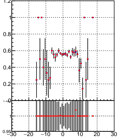
Efficiency vs sim PV z — DQM_TT_mkFit-DQM_time_orig2 — DQM_TT_mkFit-DQM_time_mod2
