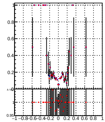
—●— DQM_TT_mkFit-DQM_time_orig2 —●— DQM_TT_mkFit-DQM_time_mod2
