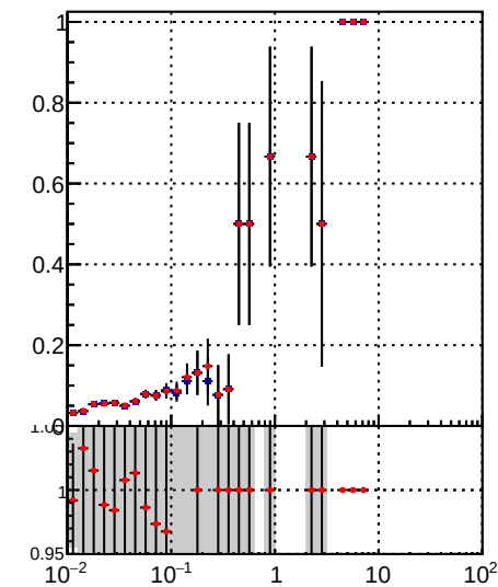
—•— DQM_TT_mkFit-DQM_time_orig2 —•— DQM_TT_mkFit-DQM_time_mod2
