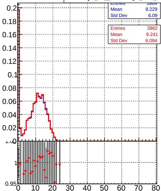
Legend: DQM_TT_mkFit-DQM_time_orig2 (grey histogram) DQM_TT_mkFit-DQM_time_mod2 (red line with points)
