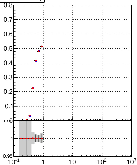
■ DQM_TT_mkFit-DQM_pless_orig ● DQM_TT_mkFit-DQM_pless_mod
