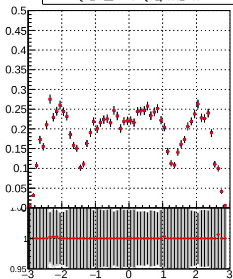
■ DQM_TT_mkFit-DQM_pless_orig ● DQM_TT_mkFit-DQM_pless_mod
