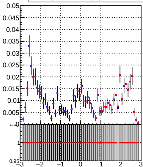
— DQM_TT_mkFit-DQM_pless_orig — DQM_TT_mkFit-DQM_pless_mod
