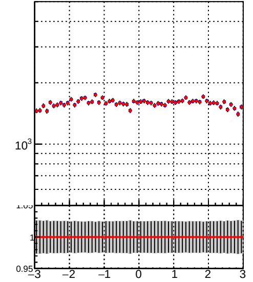
N of simulated tracks vs phi Legend: DQM_TT_mkFit-DQM_pless_orig (grey band) DQM_TT_mkFit-DQM_pless_mod (red line)
