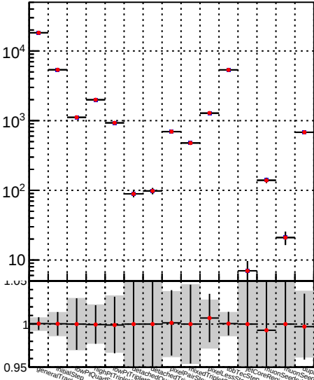
Number —●— DQM_TT_mkFit-DQM_pless_mod
