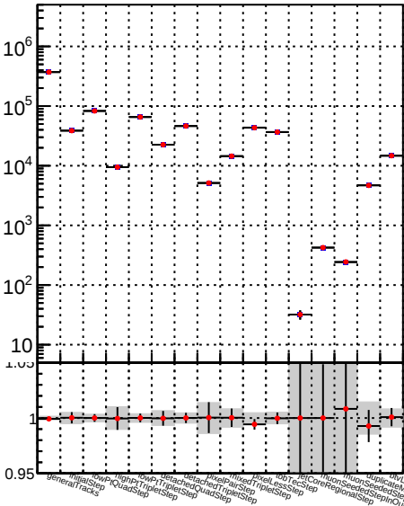
Number —●— DQM_TT_mkFit-DQM_pless_mod
