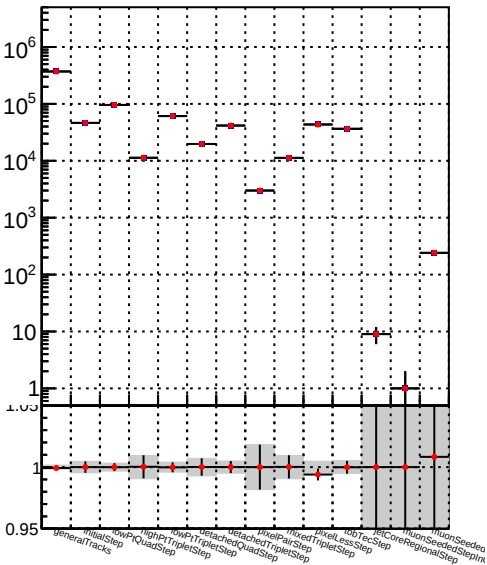
Number —●— DQM_TT_mkFit-DQM_pless_mod
