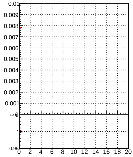
Fake rate vs. - \square - \square DQM TT mkFit-DQM_pless_orig - \bullet - \bullet DQM TT mkFit-DQM_pless_mod
