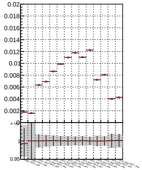
Fake rate vs. - \square - \square DQM TT mkFit-DQM_pless_orig - \bullet - \bullet DQM TT mkFit-DQM_pless_mod
