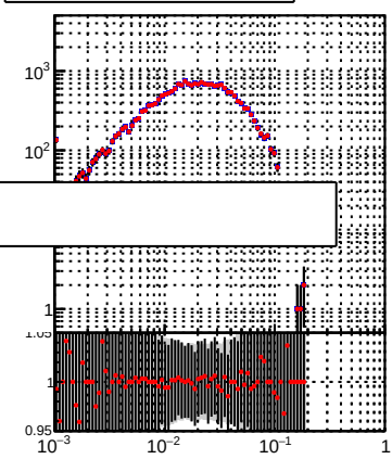
N of associated tracks (recoToSim) looped tracks vs dR
