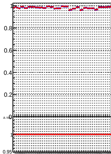
Fake rate vs. Legend for Fake rate vs. plot: Black line with blue dots: DQM TT mkFit-DQM_pless_orig Red line with red dots: DQM TT mkFit-DQM_pless_mod
