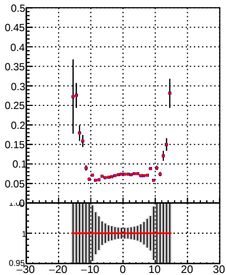
Fake rate vs d —•— DQM_TT_mkFit-DQM_pless_orig —•— DQM_TT_mkFit-DQM_pless_mod
