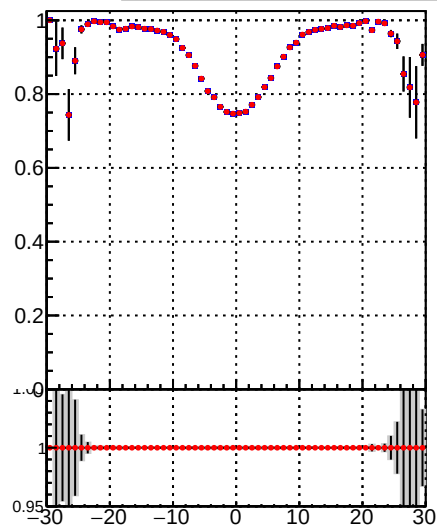
—•— DQM_TT_mkFit-DQM_pless_orig —•— DQM_TT_mkFit-DQM_pless_mod
