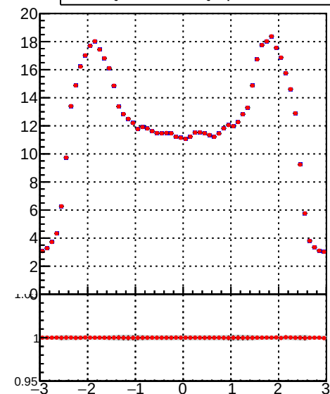
mean hit Legend: DQM_TT_mkFit-DQM_pless_orig (blue line), DQM_TT_mkFit-DQM_pless_mod (red line)
