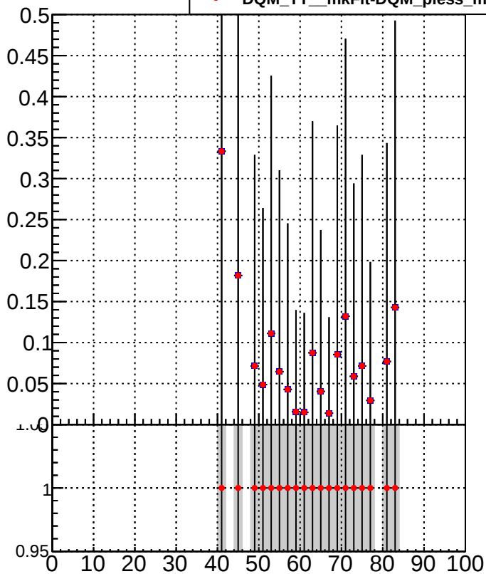
■ DQM_TT_mkFit-DQM_pless_orig ● DQM_TT_mkFit-DQM_pless_mod
