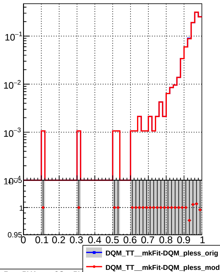
RecoPVAssoc2GenPVMatched_Missing
