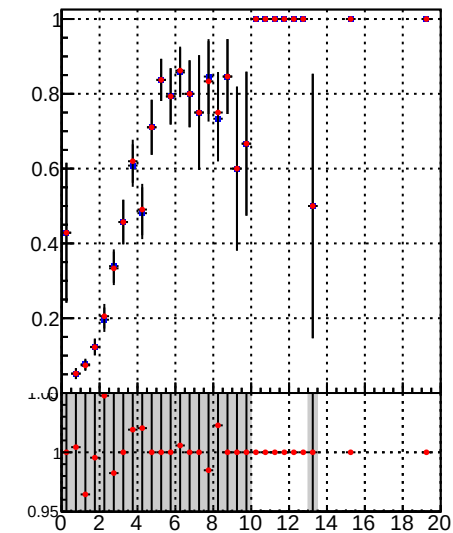
Fake rate vs. —●— DQM_TT_mkFit-DQM_pless_orig —●— DQM_TT_mkFit-DQM_pless_mod
