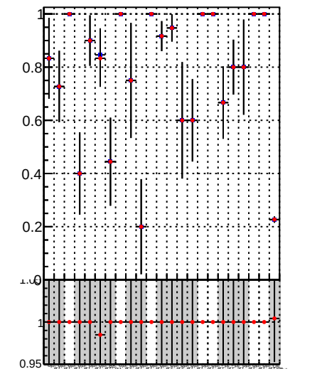
Fake rate vs. —●— DQM_TT_mkFit-DQM_pless_orig —●— DQM_TT_mkFit-DQM_pless_mod
