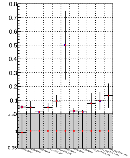
Fake rate vs. \square DQM TT mkFit-DQM_pless_orig \bullet DQM TT mkFit-DQM_pless_mod
