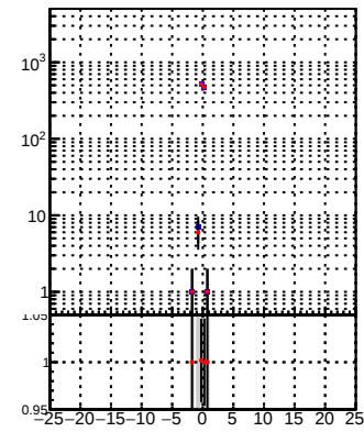
Legend: DQM_TT_mkFit-DQM_pless_orig (grey bars) DQM_TT_mkFit-DQM_pless_mod (red line)
