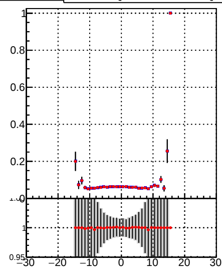
—•— DQM_TT_mkFit-DQM_pless_orig —•— DQM_TT_mkFit-DQM_pless_mod
