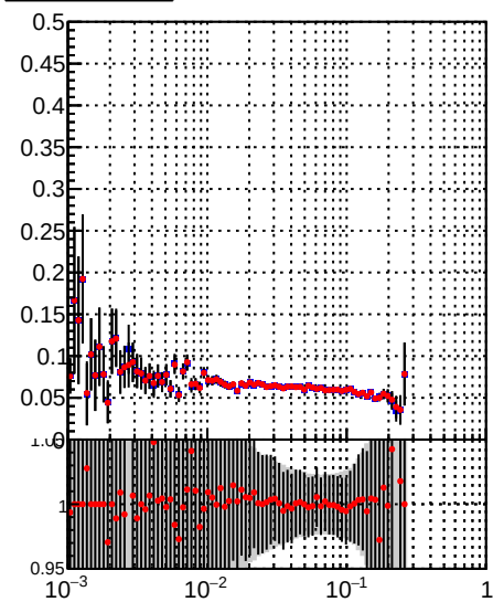
—•— DQM_TT_mkFit-DQM_pless_orig —•— DQM_TT_mkFit-DQM_pless_mod
