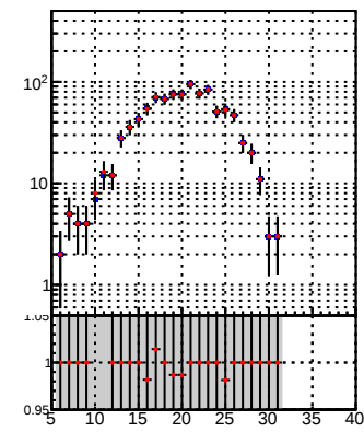
—•— DQM_TT_mkFit-DQM_pless_orig —•— DQM_TT_mkFit-DQM_pless_mod
