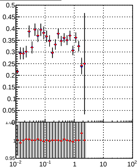
—•— DQM_TT_mkFit-DQM_pless_orig —•— DQM_TT_mkFit-DQM_pless_mod
