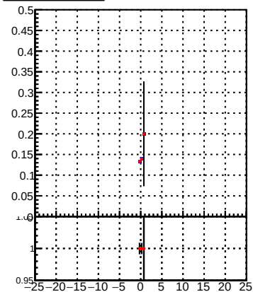
—●— DQM_TT_mkFit-DQM_pless_orig —●— DQM_TT_mkFit-DQM_pless_mod
