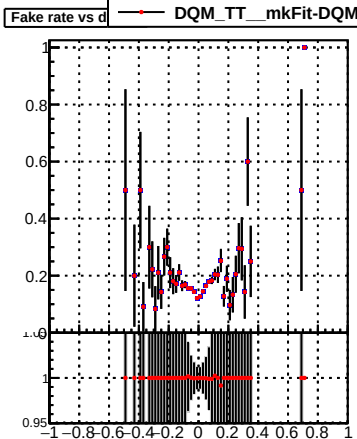
—●— DQM_TT_mkFit-DQM_pless_orig —●— DQM_TT_mkFit-DQM_pless_mod
