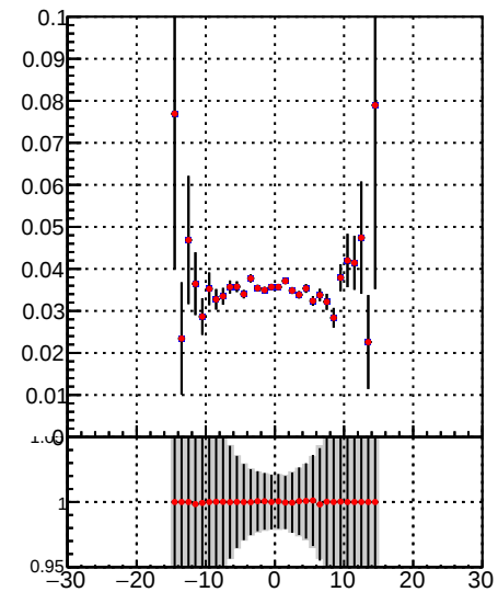
Fake rate vs d —•— DQM_TT_mkFit-DQM_pless_orig —•— DQM_TT_mkFit-DQM_pless_mod
