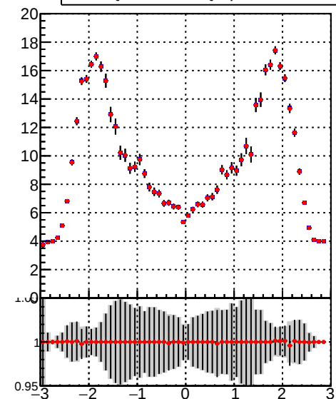
— DQM_TT_mkFit-DQM_pless_orig — DQM_TT_mkFit-DQM_pless_mod
