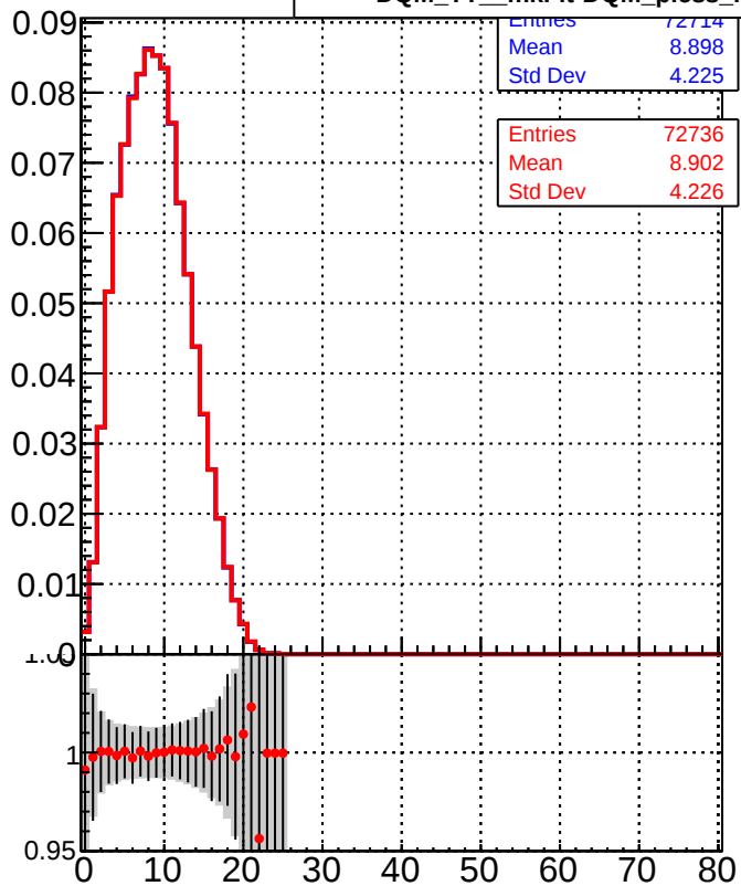
Legend: DQM_TT_mkFit-DQM_pless_orig (Blue line with squares) DQM_TT_mkFit-DQM_pless_mod (Red line with circles)
