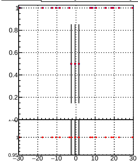
Fake rate vs v Legend: DQM_TT_mkFit-DQM_pless_orig (grey bars) DQM_TT_mkFit-DQM_pless_mod (red dots)
