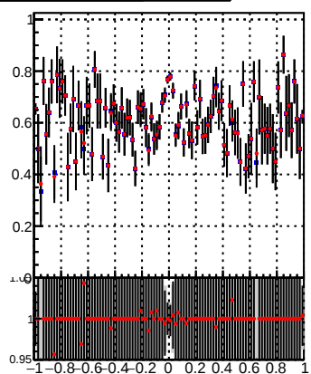
DQM_TT_mkFit-DQM_pless_mod
