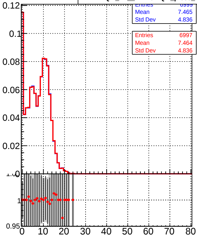
Legend: DQM_TT_mkFit-DQM_pless_orig (Blue line with squares) DQM_TT_mkFit-DQM_pless_mod (Red line with circles)
