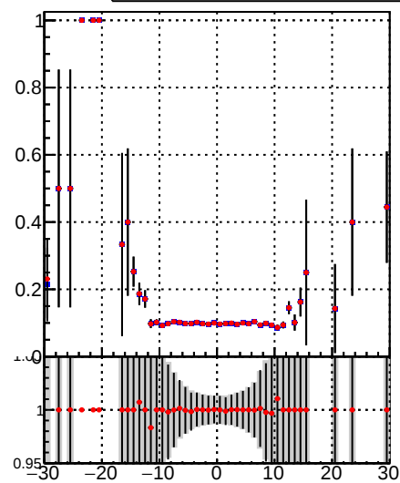
—•— DQM_TT_mkFit-DQM_pless_orig —•— DQM_TT_mkFit-DQM_pless_mod
