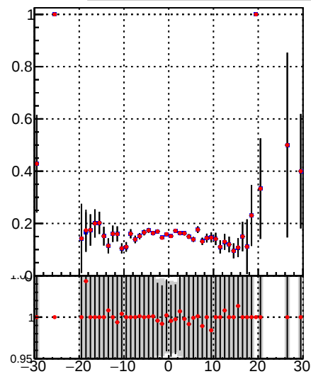
—•— DQM_TT_mkFit-DQM_pless_orig —•— DQM_TT_mkFit-DQM_pless_mod
