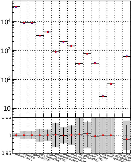
Number —●— DQM_TT_mkFit-DQM_pless_mod
