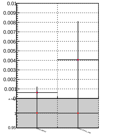
Fake rate vs. — \bullet DQM TT mkFit-DQM_pless_orig — \bullet DQM TT mkFit-DQM_pless_mod
