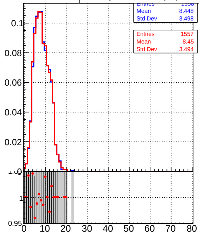
Legend: DQM_TT_mkFit-DQM_pless_orig (grey histogram, blue line with squares) DQM_TT_mkFit-DQM_pless_mod (red line with circles)
