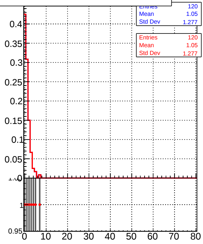
Legend: DQM_TT_mkFit-DQM_pless_orig (grey shaded area), DQM_TT_mkFit-DQM_pless_mod (red line plot)
